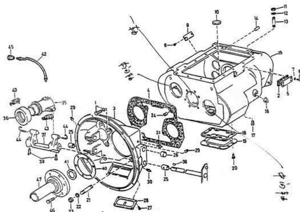
变速器RT11509C图2
